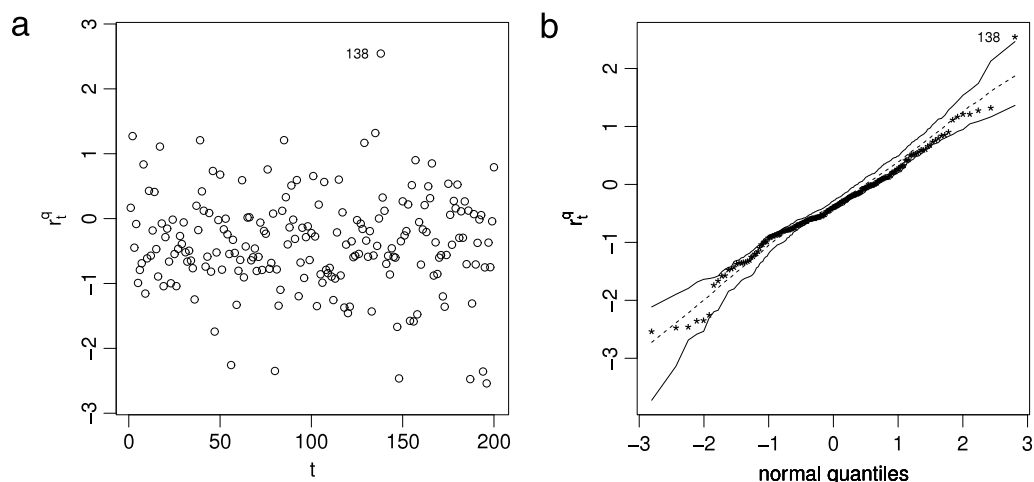
Fig. 2. Quantile residual plots.
